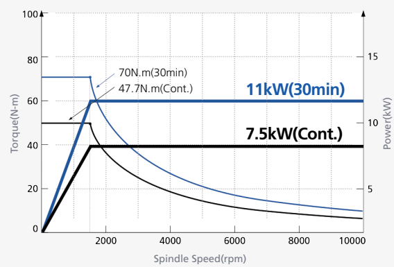
VESTA-610D (Through-spindle)
